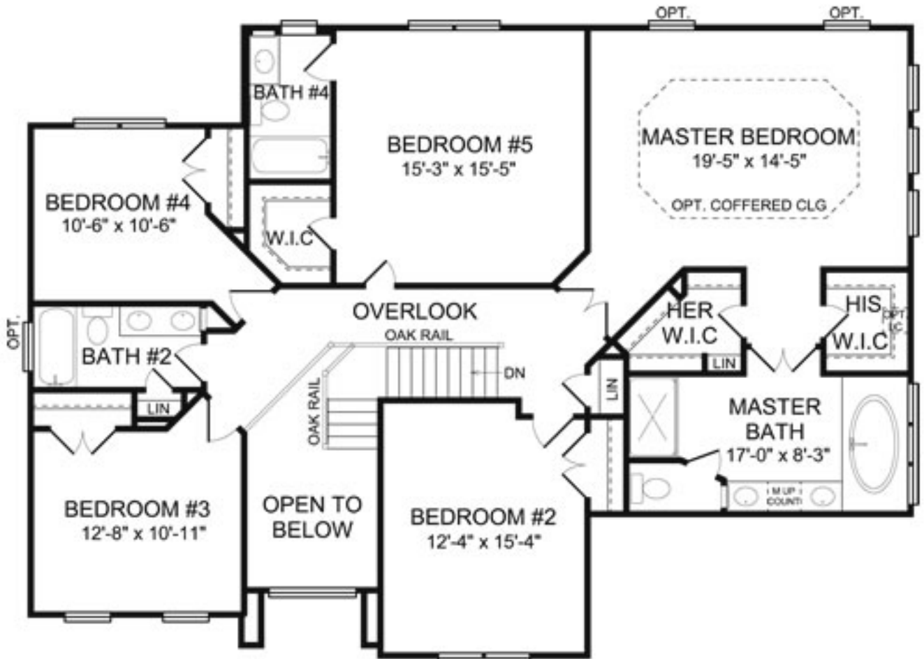
SECOND FLOOR PLAN THE YORKSHIRE MANOR
